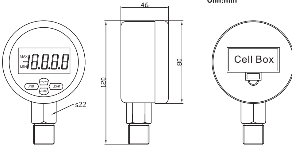
MD-S280 INTELLIGENT PRESSURE GAUGE(Dial Diameter 80mm)
