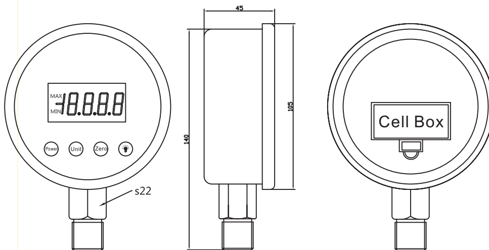
MD-S200 INTELLIGENT PRESSURE GAUGE ( Dial Diameter100mm )
